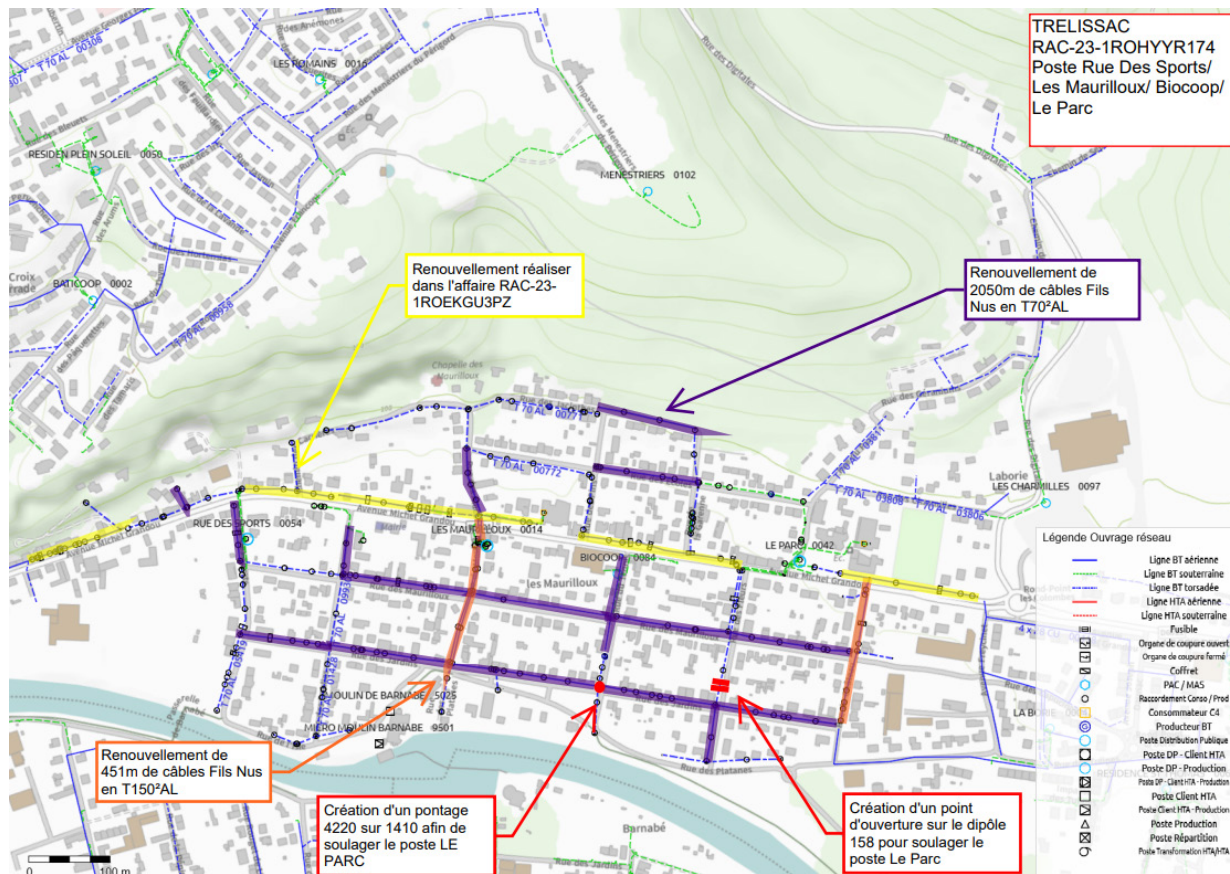
Plan solution coordination BT Trélassac
